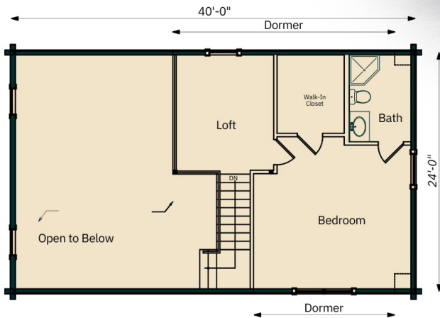
SECOND FLOOR
