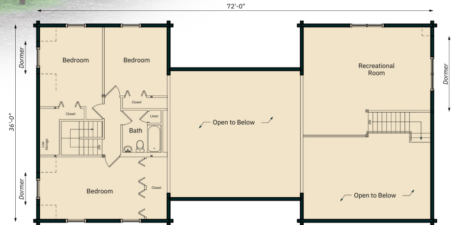
SECOND FLOOR
