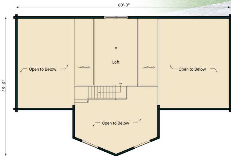
SECOND FLOOR
