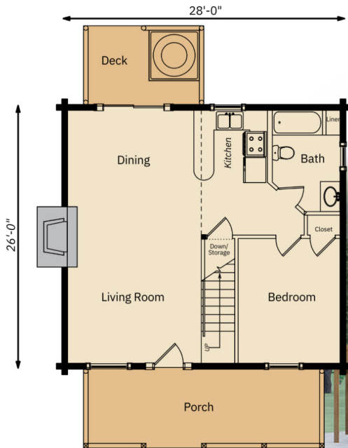
MAIN FLOOR
