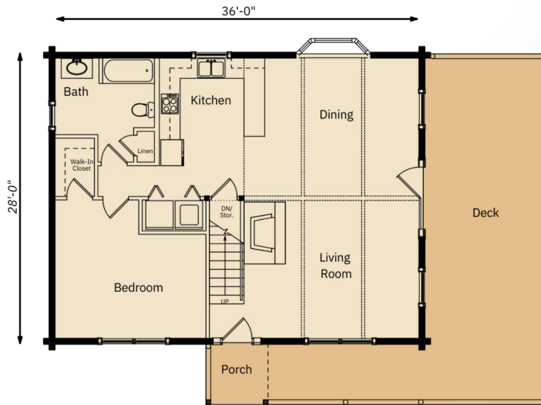
MAIN FLOOR
