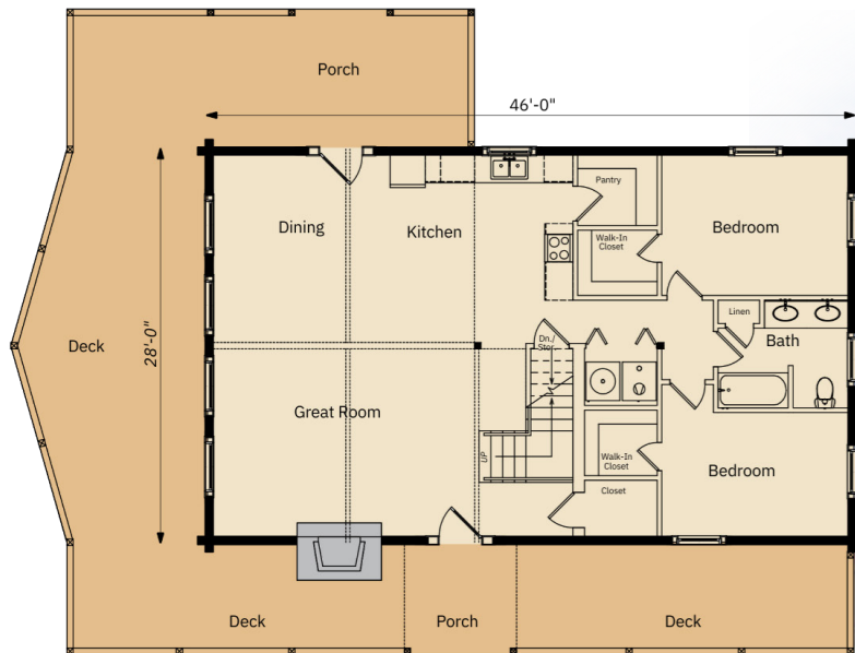
MAIN FLOOR
