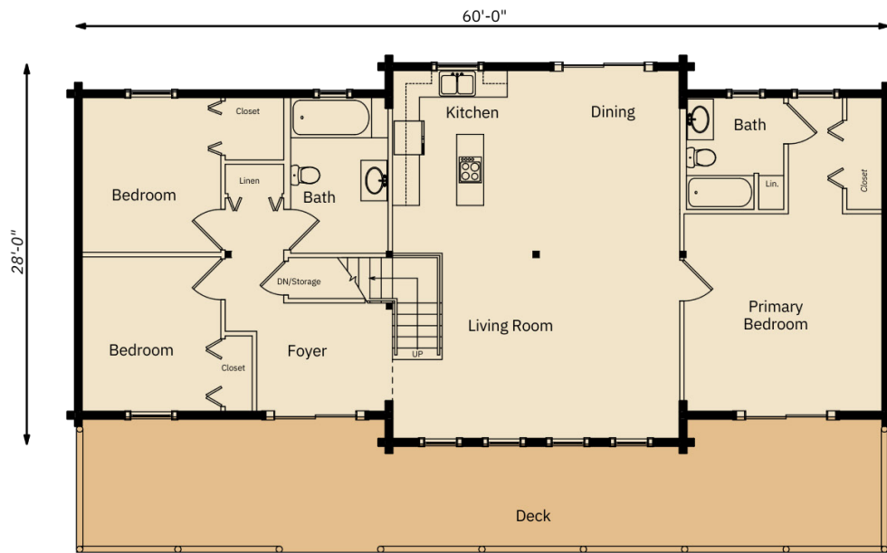
MAIN FLOOR
