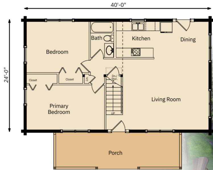
MAIN FLOOR
