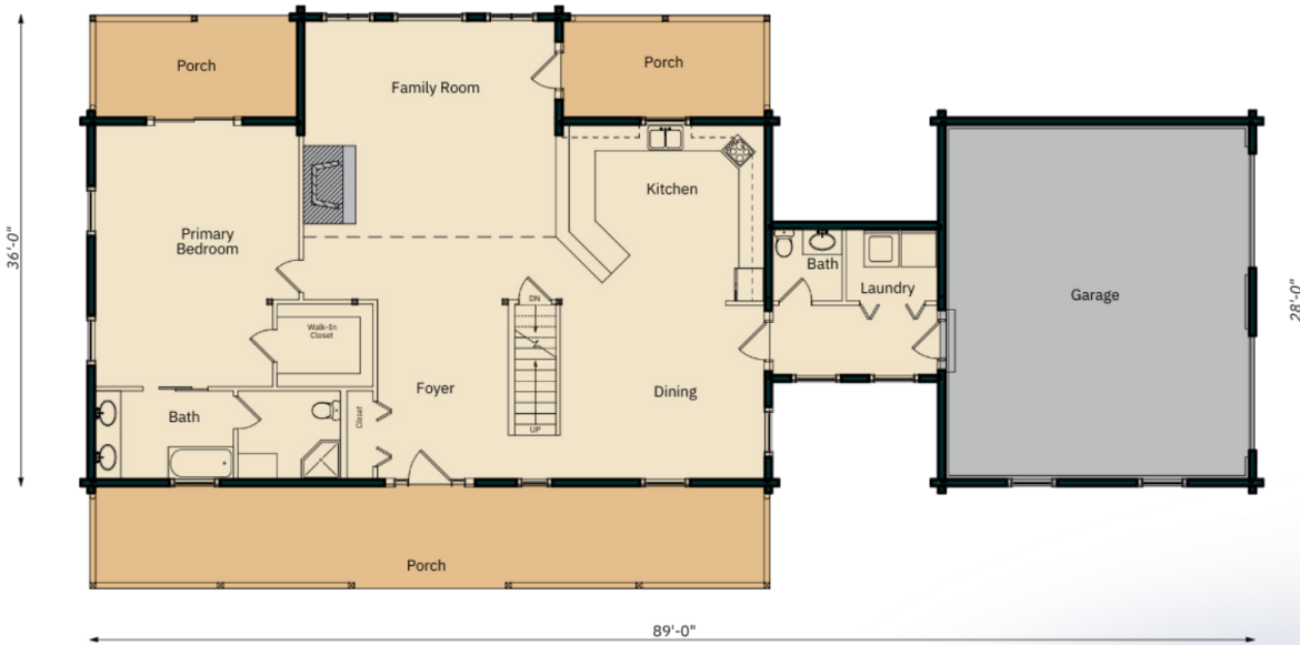
MAIN FLOOR
