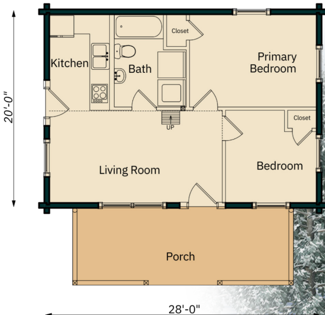
MAIN FLOOR
