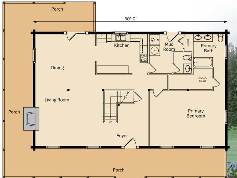
MAIN FLOOR
